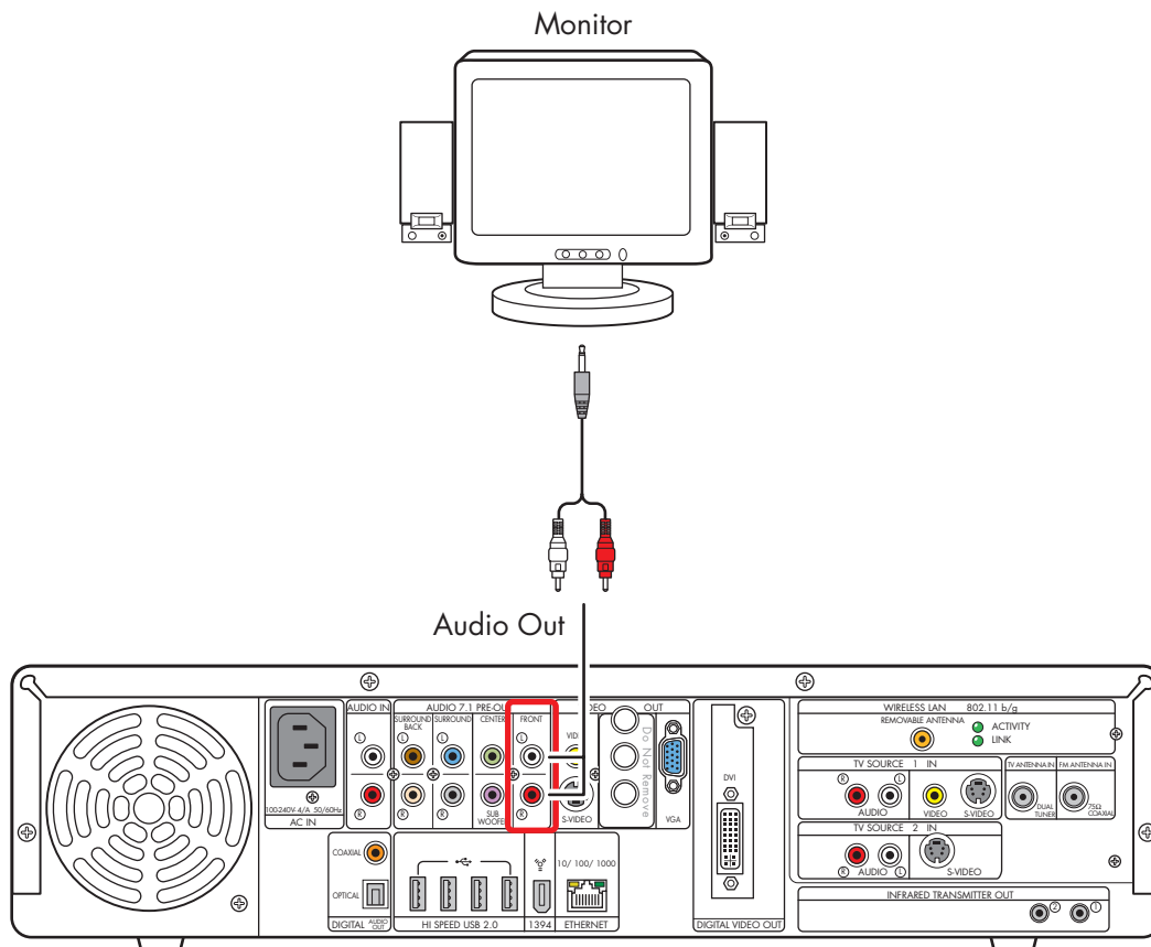
Monitor speaker installation (2.0 shown)
